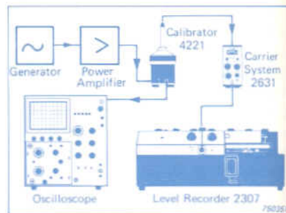
Fig. 6. Set-up for recording low frequency response of microphones
