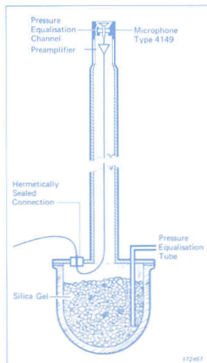
Fig. 2. The dehumidification system
